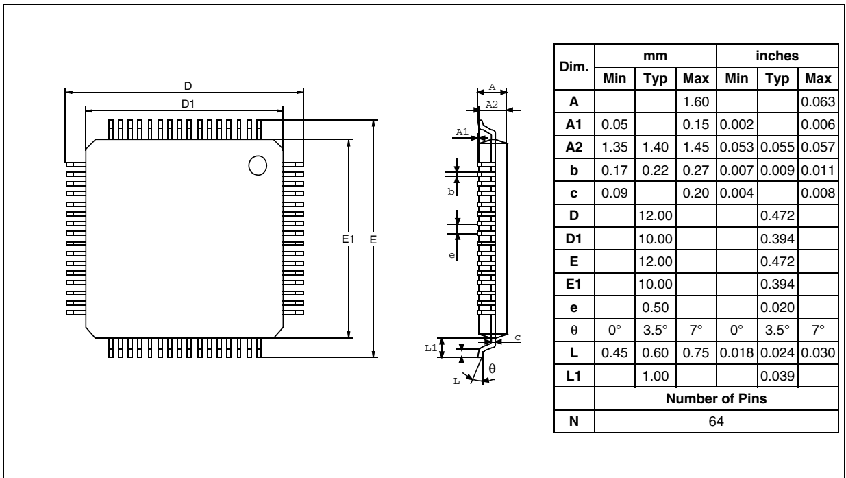
Figure 149. 64-Pin Low Profile Quad Flat Package (10 x10)
