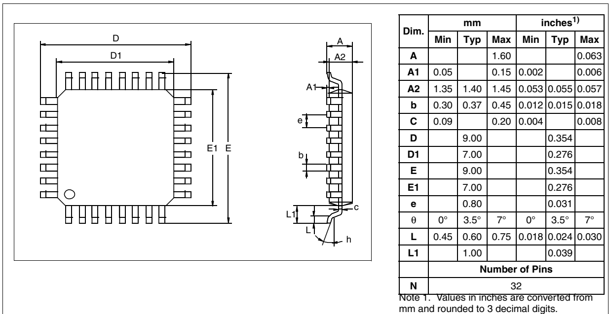
Figure 147. 32-Pin Low Profile Quad Flat Package (7x7)
