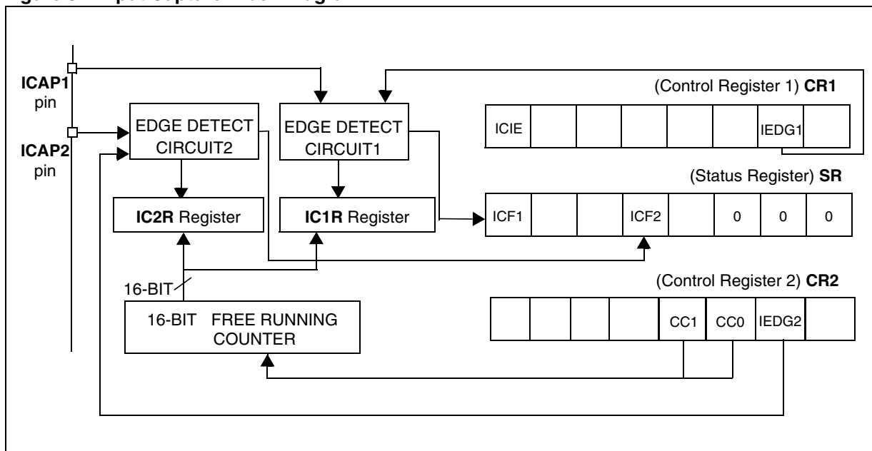
Figure 52. Input Capture Block Diagram
