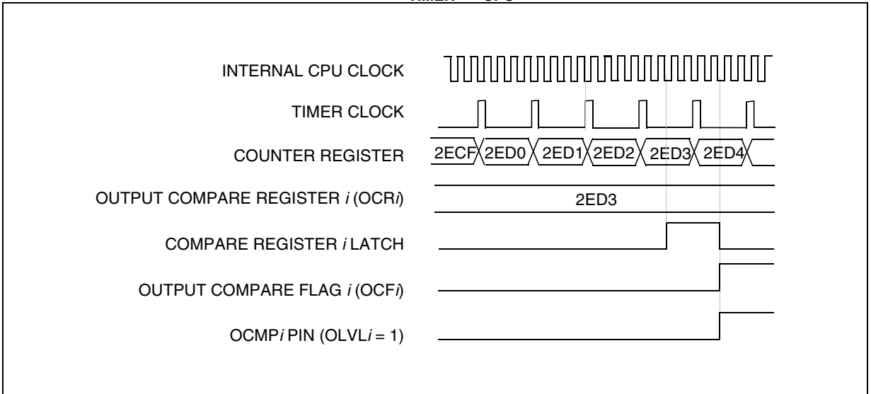
Figure 56. Output Compare Timing Diagram, f_{TIMER} = f_{CPU}/4
